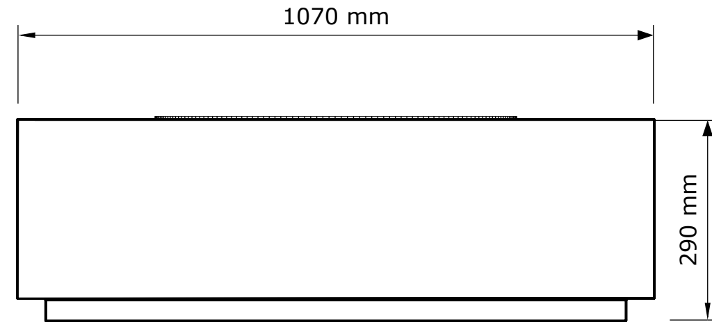
Front View
